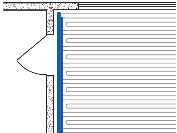
Pipe routing plan with welded saddle
