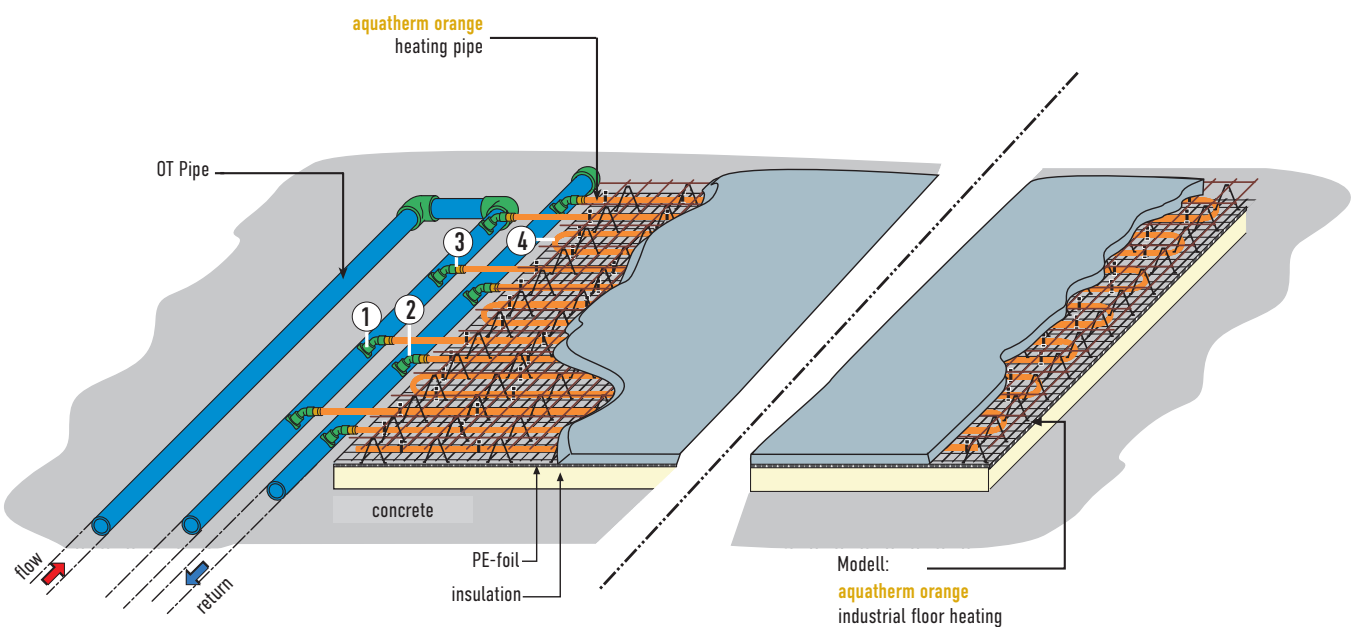
Pipe routing plan with welded saddle
